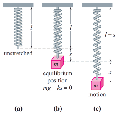
FIGURE 5.1.1 Spring/mass system
