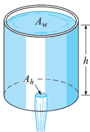
FIGURE 1.3.3 Draining tank
