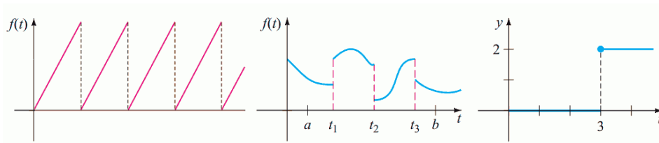
Like operator of differentiation converts function f(x) into other function f'(x) , so the Laplace operator converts functions. By means of Laplace operator discontinuous function can be converted into other function.
