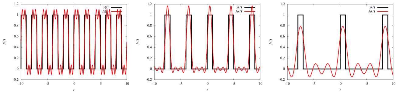
Approximation of the square function by three terms of Fourier series ( n = 3 ).
