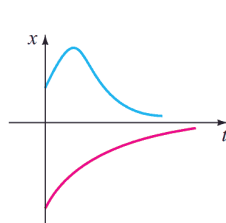
FIGURE 5.1.7 Motion of a critically damped system
