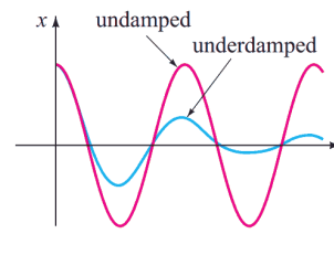
FIGURE 5.1.8 Motion of an underdamped system
