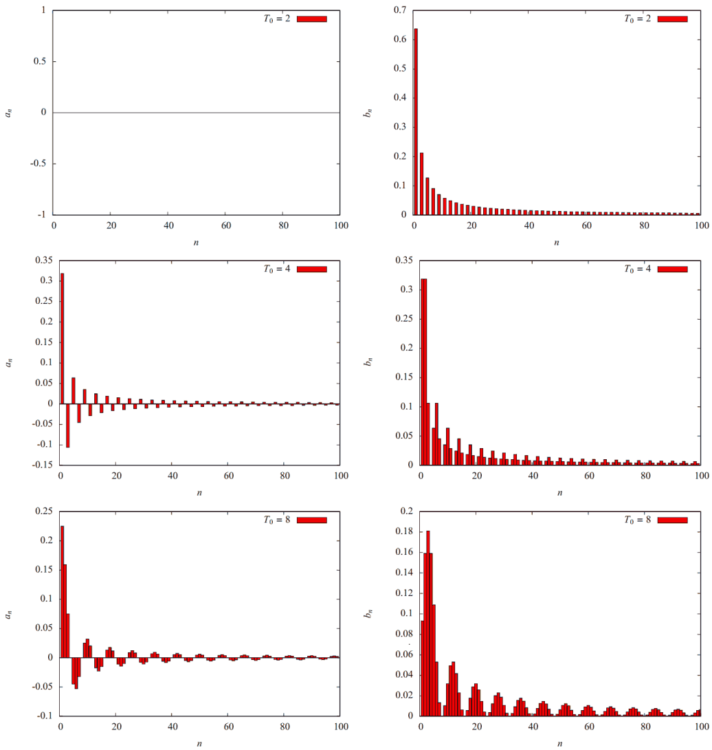
First one hundred coefficients a_1, a_2, \dots, a_{100} of cosines (on the left) and b_1, b_2, \dots, b_{100} for sines (on the right).
