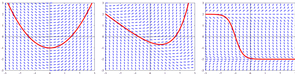
Differential equations drawn as a direction field for three different DE. Also one particular solution drawn in red color for each.
