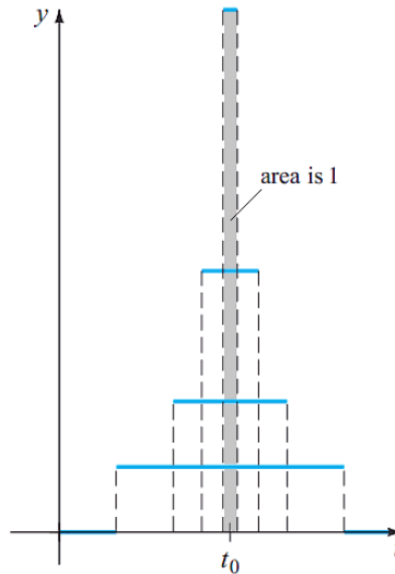
FIGURE 7.5.2 Unit impulse
